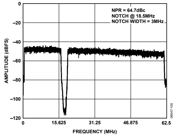
Figure 38. AD9640 Noise Power Ratio (NPR)
