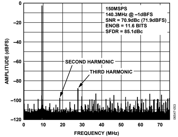
Figure 19. AD9640-150 Single Tone FFT with f_{IN} = 140.3 MHz
