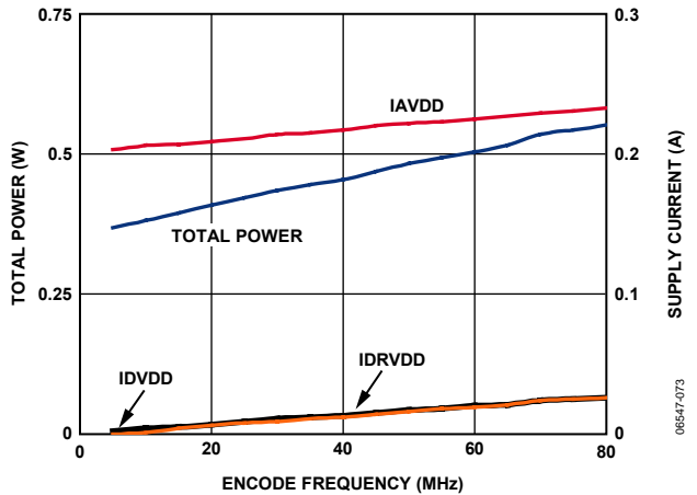
Figure 66. AD9640-80 Power and Current vs. Clock Frequency
