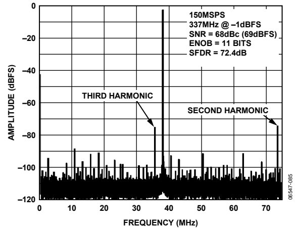
Figure 21. AD9640-150 Single Tone FFT with f_{IN} = 337 MHz
