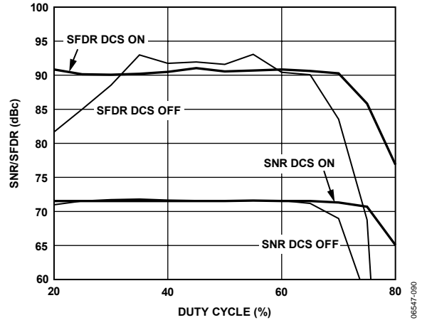
Figure 43. AD9640 SNR/SFDR vs. Duty Cycle with f_{IN} = 10.3 MHz
