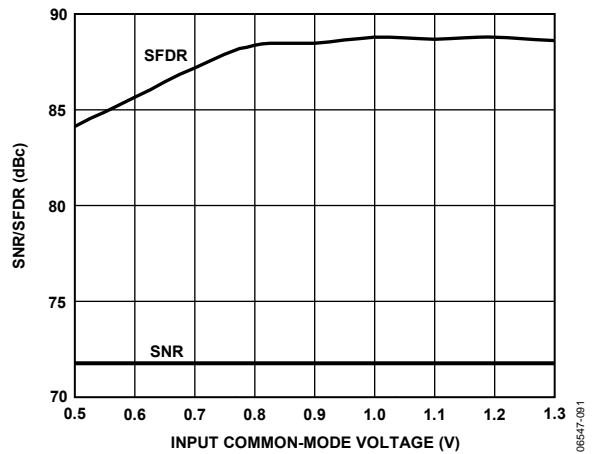
Figure 44. AD9640 SNR/SFDR vs. Input Common Mode (VCM) with f_{IN} = 30 MHz
